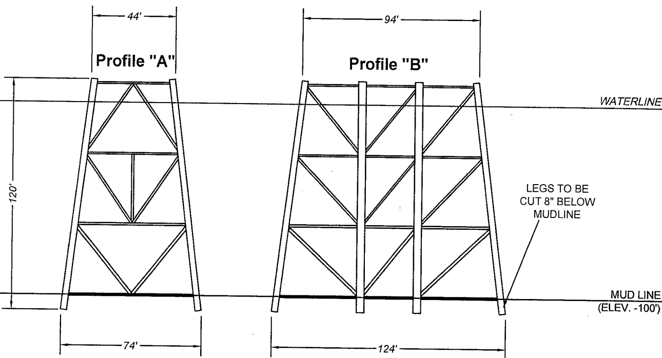
PROFILES "A" & "B" (note: 1 structure, 2 aspects) (PRE-DEPLOYMENT)
