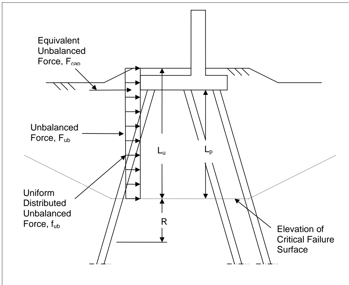
Figure 3. Unbalanced Forces.
