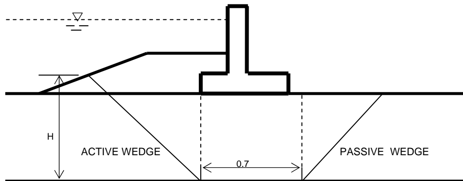
Figure 1. Typical Failure Plane Beneath a T-Wall
