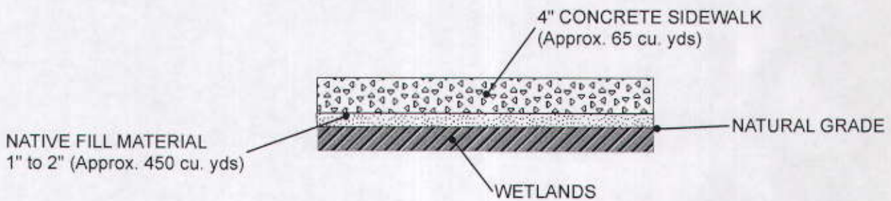
TYPICAL CLUBHOUSE PARKING AREA SECTION NOT TO SCALE
