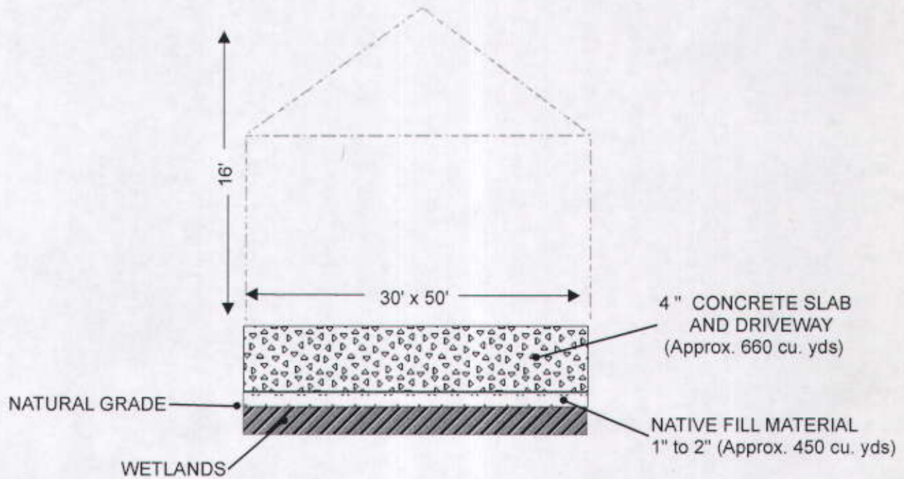
TYPICAL CONCRETE CLUBHOUSE SLAB SECTION NOT TO SCALE
